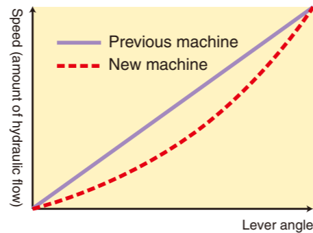
Attachment lever touch
